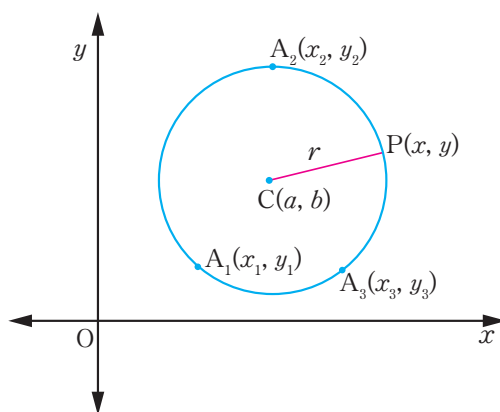
Figure 4.15: Three points on a circle
