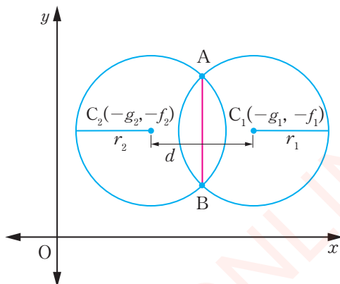
Figure 4.20: Circles intersecting at two distinct points
