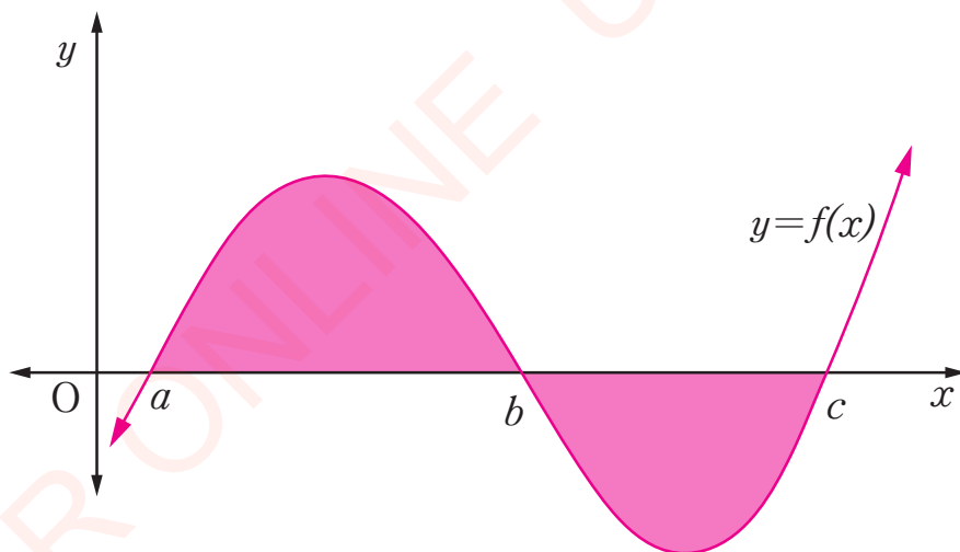
Figure 10.5: Area under a curve
