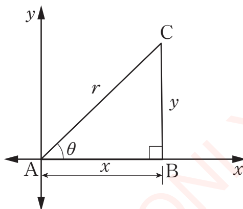
Figure 7.2: A right-angled triangle in the xy -plane
