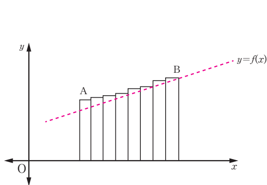
Figure 10.12(a): Slices of a rotated solid
