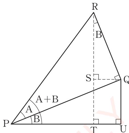
Figure 7.3: Illustrative sketch for deriving compound angle formulae
