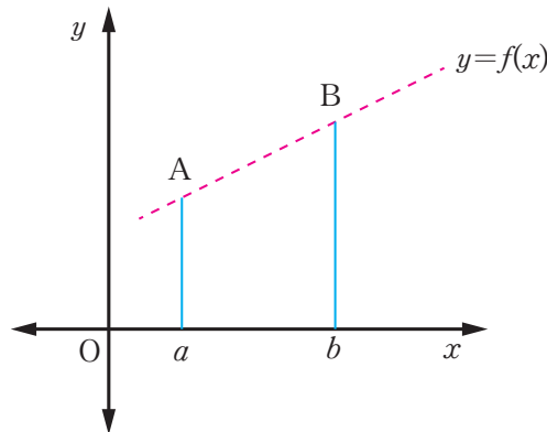
Figure 10.10 (a): The curve and its boundaries
