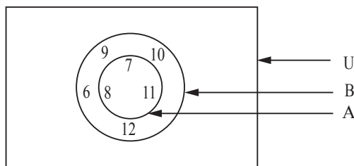
Figure 2.4: Subsets in a Venn diagram
