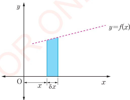
Figure 10.11(a): Thin strip of the plain
