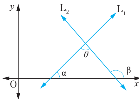
Figure 4.7: Angle of intersection between two lines L_1 and L_2
