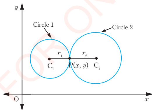
Figure 4.18: Two circles intersecting externally
