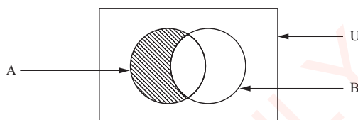
Figure 2.8: Shaded region showing the relative difference of set A with respect to set B
