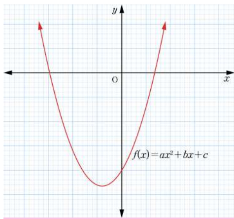
Figure 5.2(a) : Graph of a quadratic function for a > 0
