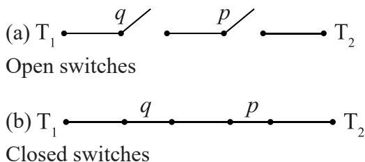
Figure 3.1 Open and closed switches in series connection
