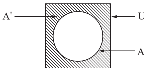
Figure 2.9: Shaded region showing A' .
