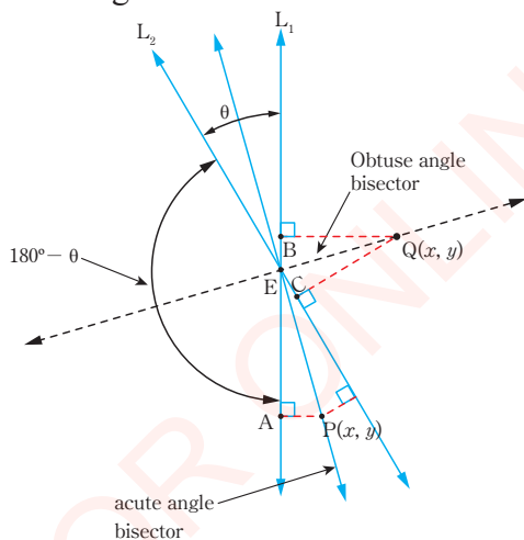
Figure 4.10: Angle bisector with lines L_1 and L_2
