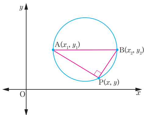
Figure 4.14: Circle with end points of a diameter
