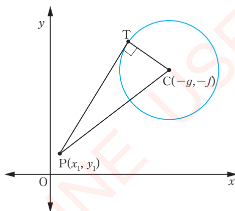
Figure 4.22: Length of a tangent from a point to a circle
