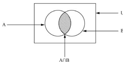
Figure 2.5: Shaded region showing the intersection of sets A and B
