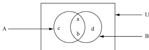
Figure 2.2: Joint sets in a Venn diagram
