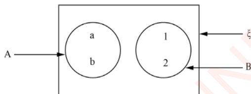
Figure 2.3: Disjoint sets in a Venn diagram
