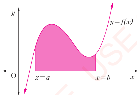
Figure 10.4: Bounded region of the function y = f(x)
