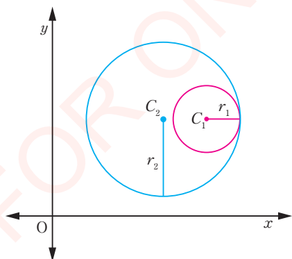
Figure 4.19: Two circles intersecting internally
