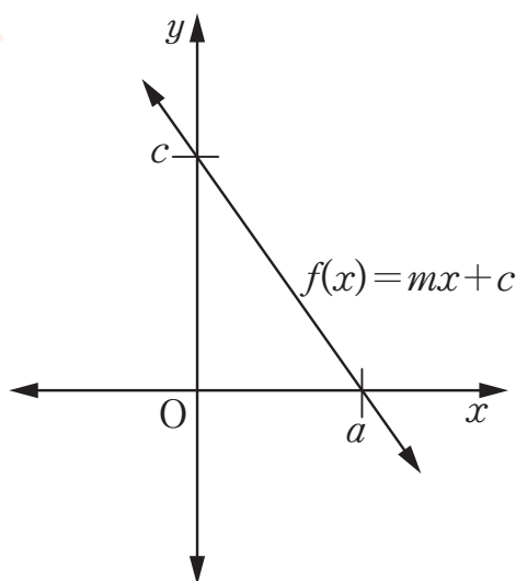
Figure 5.1: Graph of f(x) = mx + c , for m < 0
