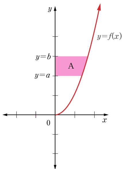
Figure 10.6: Area between a curve y = f(x) and the y-axis
