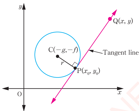
Figure 4.16: Tangent line to a circle
