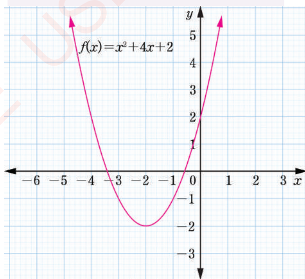
Figure 5.2(a) : Graph of a quadratic function for a > 0
