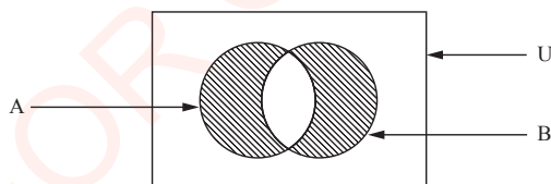
Figure 2.7: Shaded region showing the symmetric difference of sets A and B
