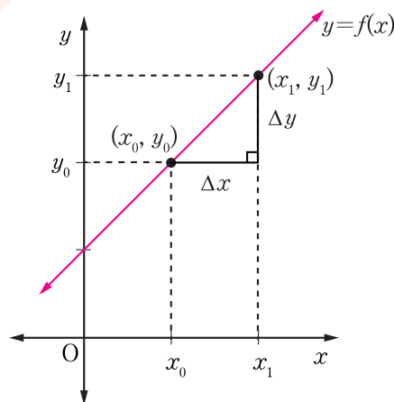
Figure 9.1: Graph of a straight line
