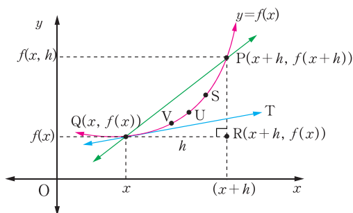
Figure 9.2: Illustration of the gradient of a curve y = f(x) between the points P(x+h, f(x+h)) and Q(x, f(x))
