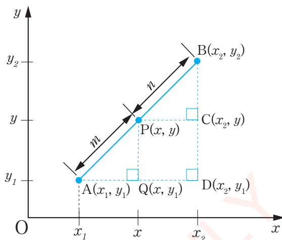
Figure 4.11: Internally division of a line
