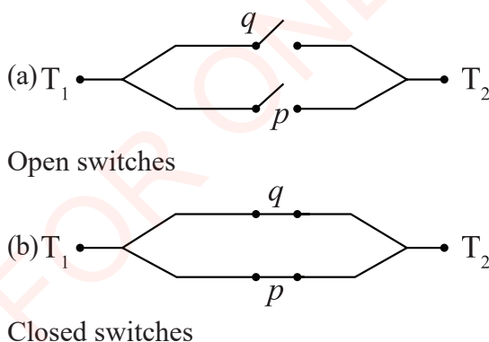
Figure 3.2: Open and closed switches in parallel connection
