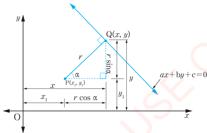
Figure 4.8: Perpendicular distance of a point from a line
