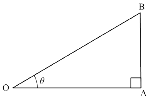
Figure 7.1: A right-angled triangle OAB
