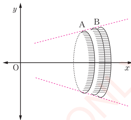
Figure 10.12(b): A rotated solid
