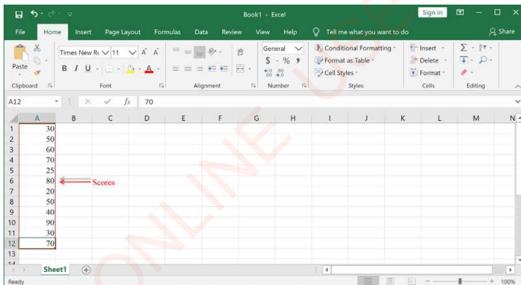
Figure 1.8: Scores of students in a certain test
