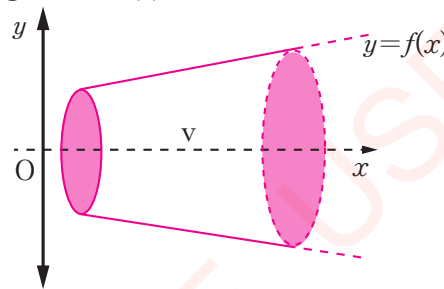
Figure 10.10 (b): Solid rotated through a complete revolution about the x -axis
