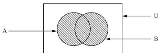
Figure 2.6: Shaded region showing the union of sets A and B
