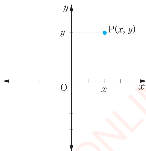
Figure 4.2: Position of the point P(x, y)
