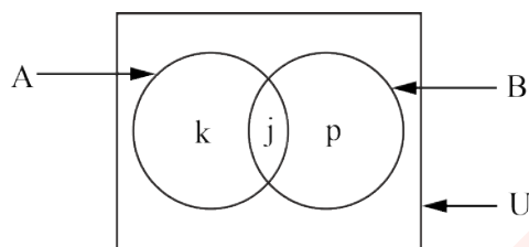
Figure 2.10: Two enclosed sets in the universal set
