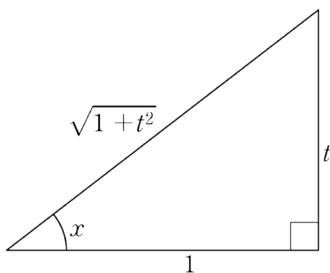
Figure 10.1: A right-angled triangle
