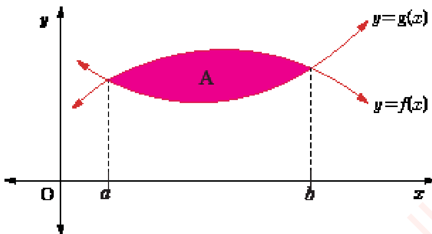
Figure 10.7: Area enclosed between two curves
