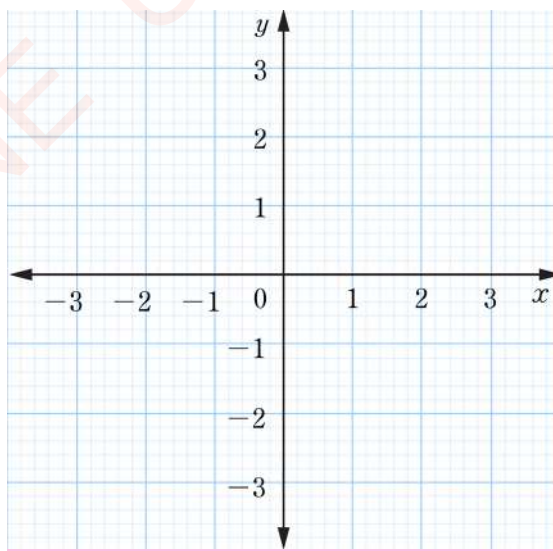
Figure 4.1: The xy - coordinate system
