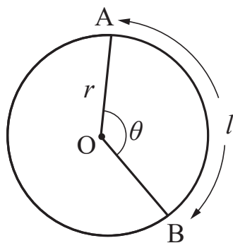
Figure 7.6: Sketch describing an arc of a circle.
