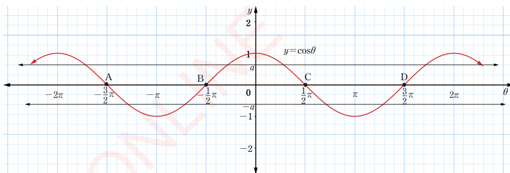
Figure 7.5: Graph of f(\theta) = \cos\theta
