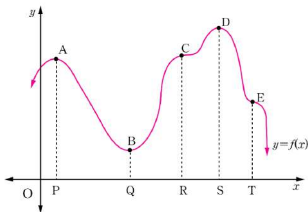
Figure 9.3: Turning points and points of inflexion
