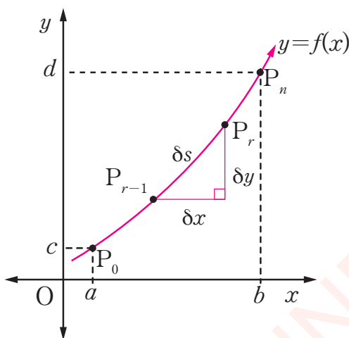
Figure 10.9: Length of an arc
