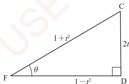
Figure 7.4: A right-angled triangle DCF
