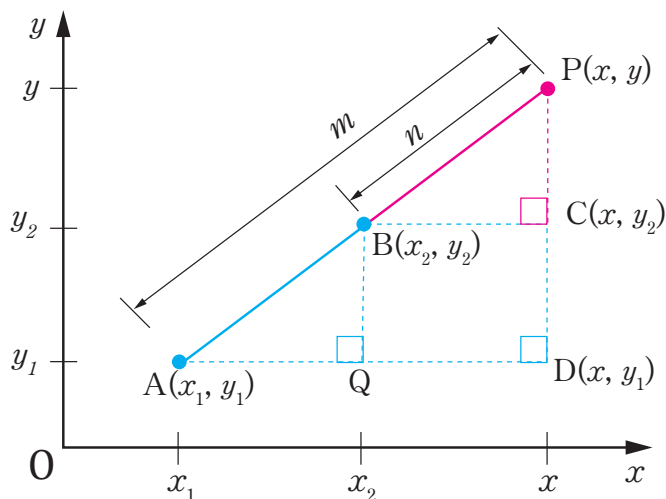
Figure 4.12: External division of a line
